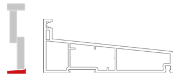
Flush Cill
