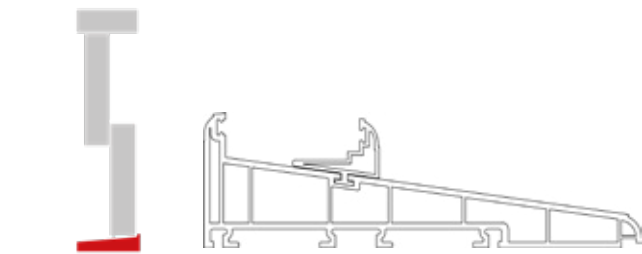
180mm Protruding Cill
